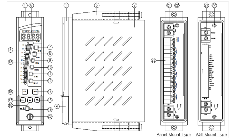
[Figure 4. Components of concentration display unit]
