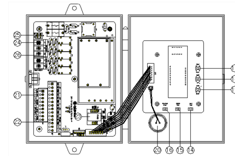
[Figure 1. GTC-520 components]
