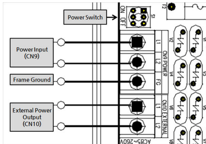
[Figure 2. Configuration of GTC-520A power supply]
