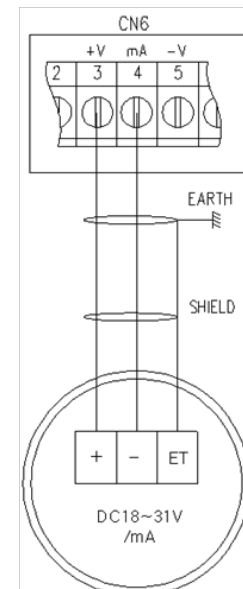
[Figure 6. 2-wire type gas detector]
