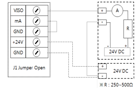
[Figure 6. 4~20mA 3 Wire Sink Driver Outline]
