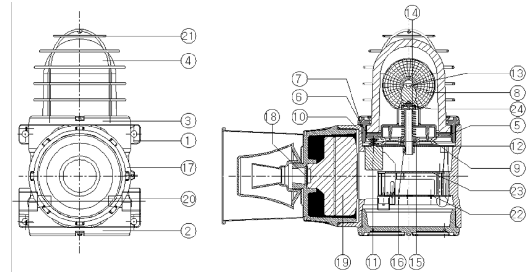
[Figure 1. Combination Type Configuration]
