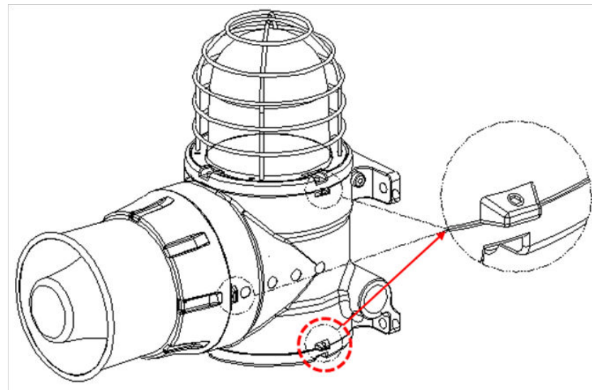
[Figure 3. Slotted Set Screw Configuration]
