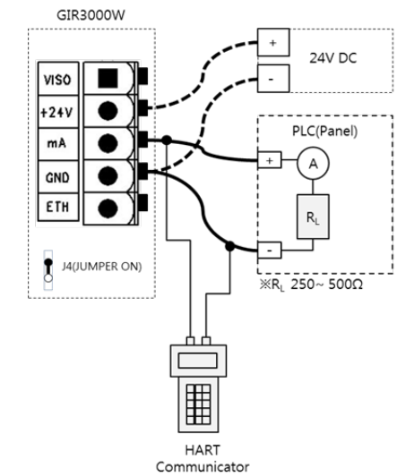
[Figure 9. Configuration of 4-20mA Source]
