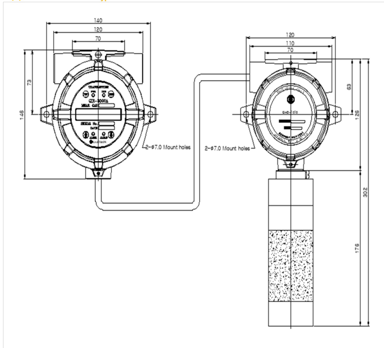
[Figure 22. GIR-3000W remote Type]
