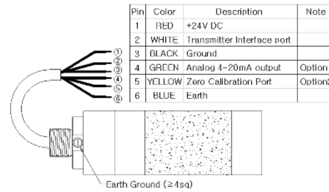
[Figure 15. Configuration of GSA920A connection]
