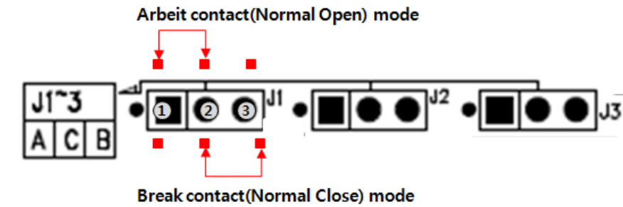
[Figure 13. Setting for Relay Mode]
