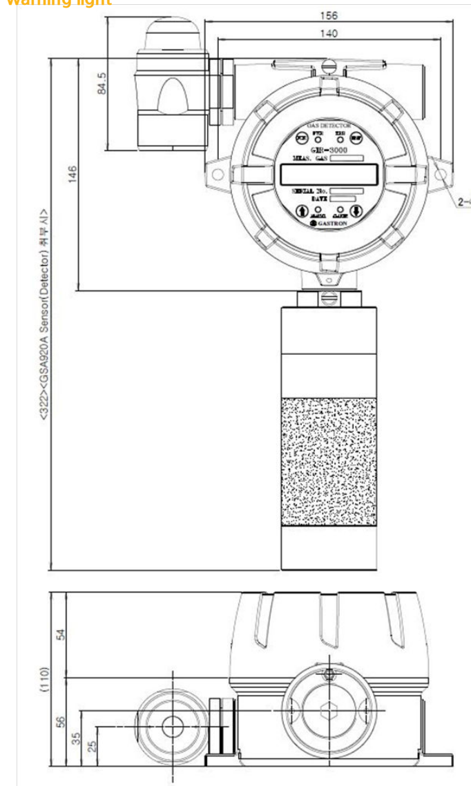
[Figure 21. Outline drawing for coupling of GIR-3000W warning light]
