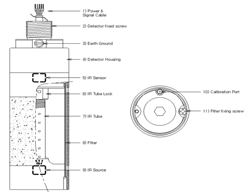
[Figure 3. Components of GIR-3000W Sensor]
