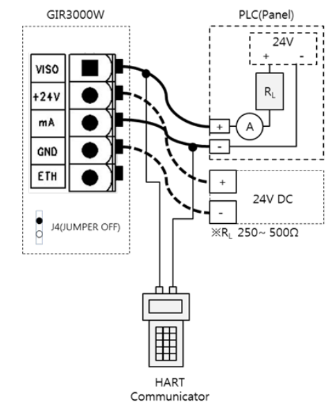
[Figure 10. Configuration of 4-20mA Sink]
