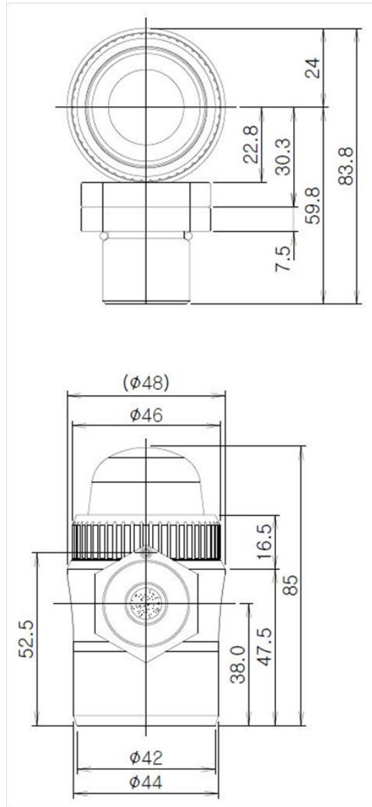
[Figure 20. Outline drawing for GTL-100]
