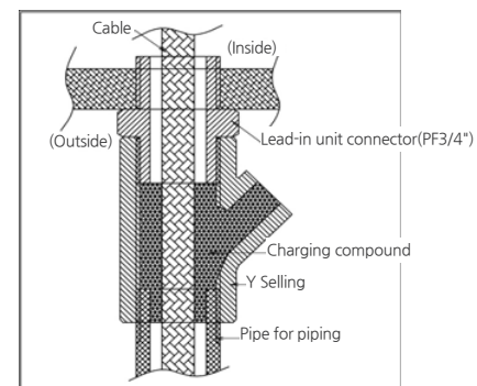
[Figure 24. Y Sealing Compound]
