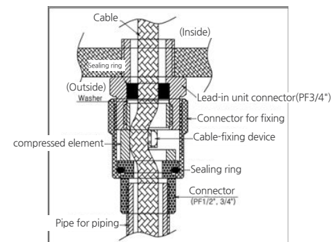
[Figure 23. Pressure-resistant lacking type]
