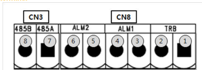
[Figure 12. Relay and RS485 Terminal]
