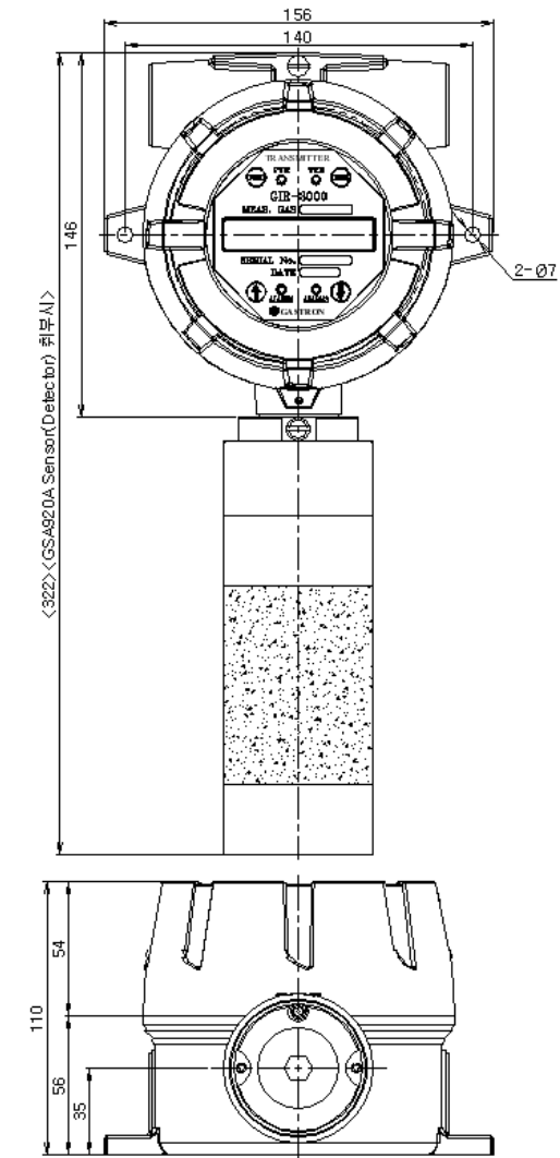
[Figure 19. Outline drawing for GIR-3000W Standard Type]
