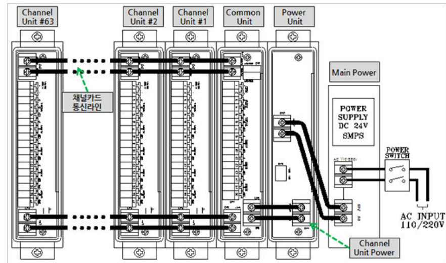
[Figure 4. Power supply and signal configuration for channel card]
