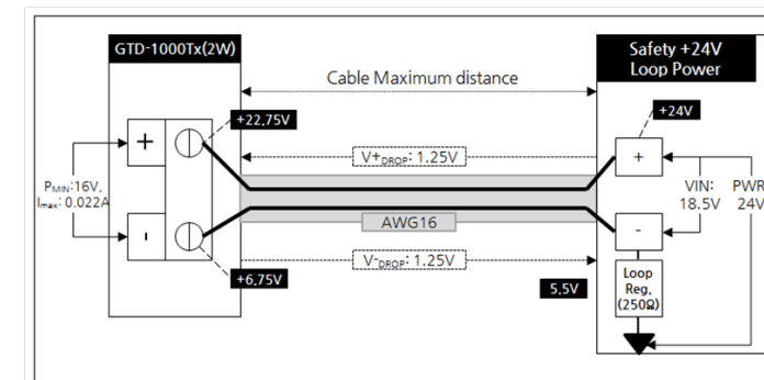
[Figure 7. Calculation of GTD-1000Tx(2W) Installation Cable Length]
