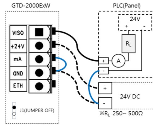
[Figure 9. 4-20mA 3Wire Sink Configuration]
