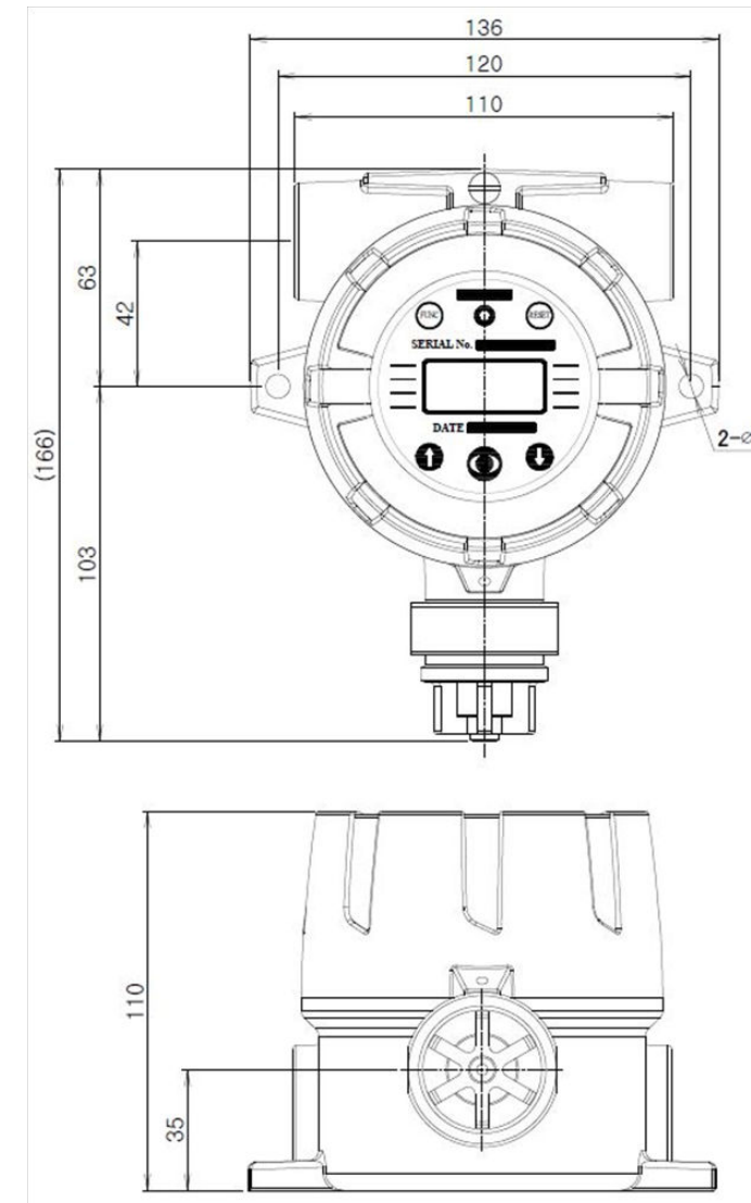
[Figure 12. GTD-2000ExW Standard Type Drawing]
