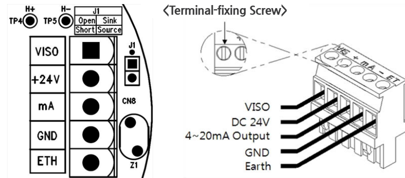
[Figure 6. CN8 Terminal Configuration]
