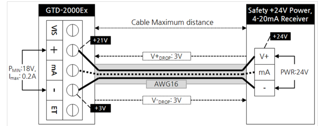
[Figure 10. Calculation of GTD-2000ExW Installation Cable Length]
