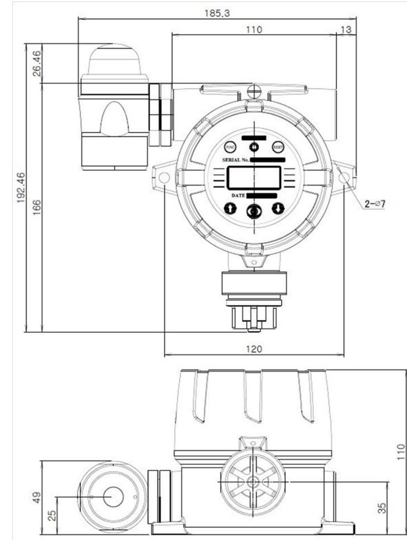
[Figure 14. GTD-2000Tx Warning Light Connection Drawing]
