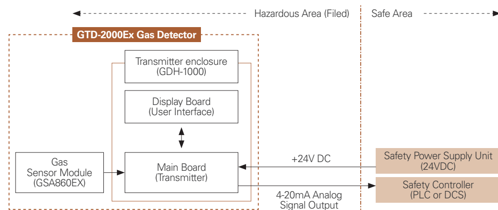
[Figure 1. GTD-2000ExW Overview]
