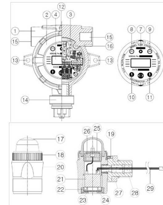
[Figure 2. GTD-2000ExW Components]
