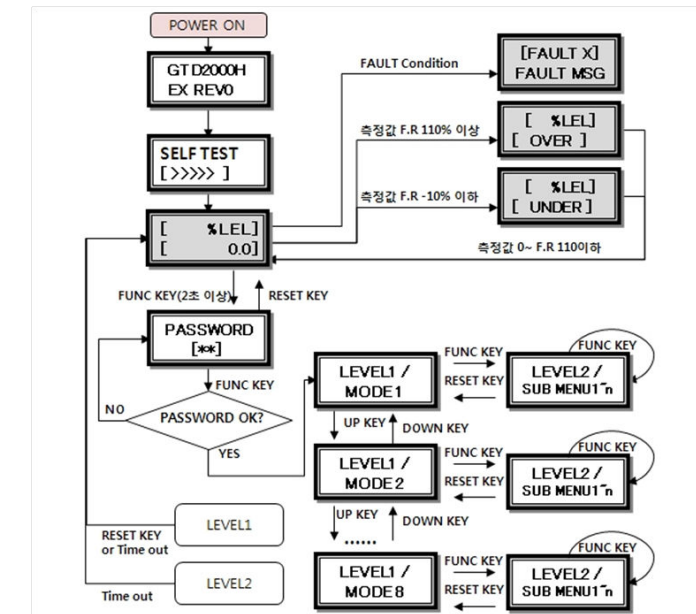
[Figure 11. GTD-2000ExW Mode Configuration]
