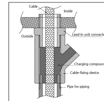
[Figure 16. Y Sealing Compound]
