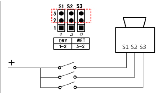
[Figure 5. Wet Contact Configuration]
