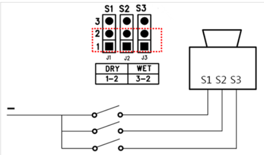
[Figure 4. Dry Contact Configuration]
